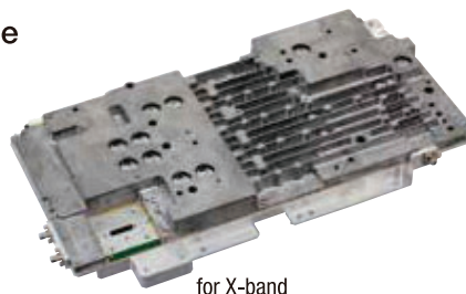
Power Amplifier Module of the Solid State transceiver
